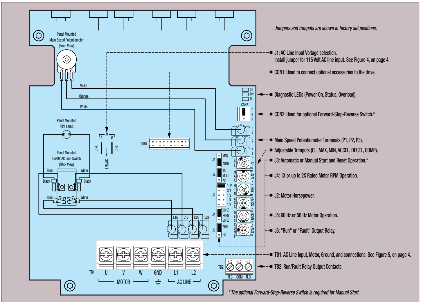
FIGURE 3 – CONTROL LAYOUT
