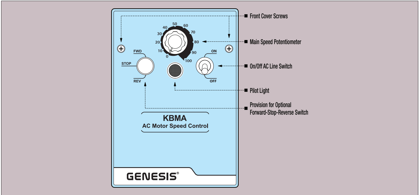
FIGURE 3 – CONTROL LAYOUT
